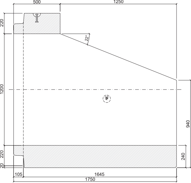
PATKOVÁ TROUBA TZP-SP 120/175/50 SD
