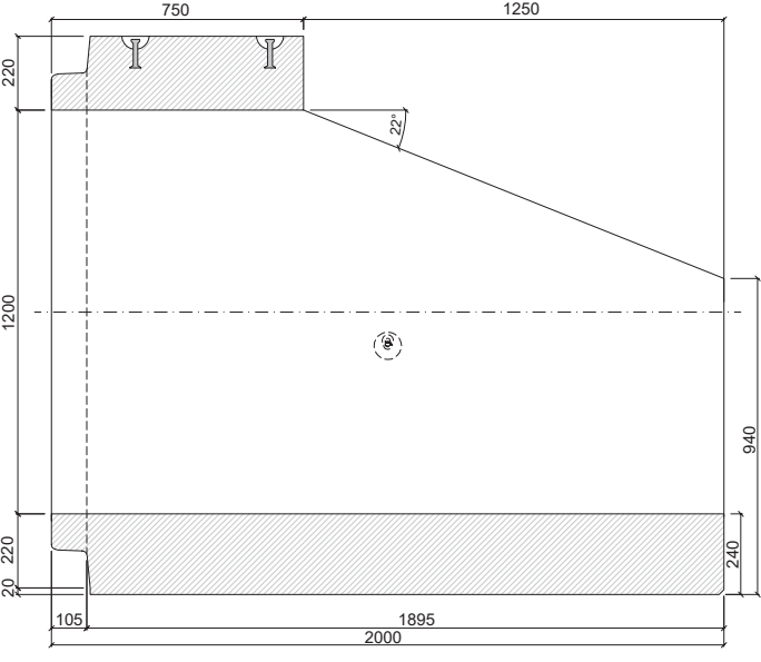
PATKOVÁ TROUBA TZP-SP 120/200/75 SD
