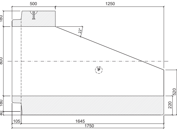
PATKOVÁ TROUBA TZP-SP 80/175/50 SD
