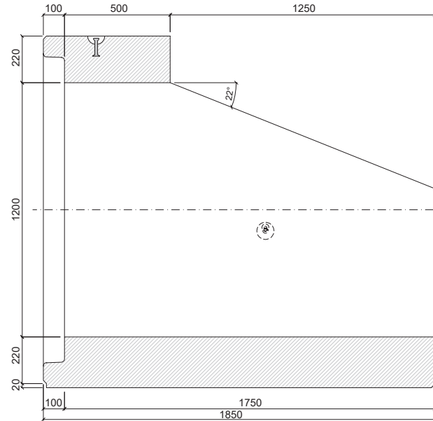
PATKOVÁ TROUBA TZP-SP 120/175/50 SH
