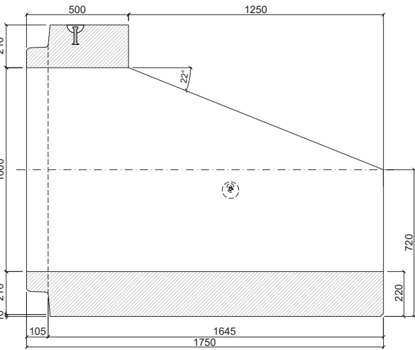
PATKOVÁ TROUBA TZP-SP 100/175/50 SD
