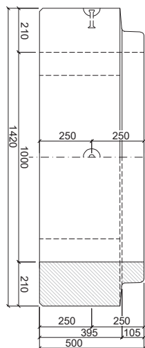
PATKOVÁ TROUBA TZP-SP 100/50 KD
