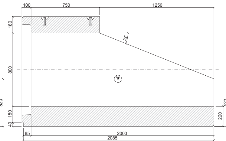
PATKOVÁ TROUBA TZP-SP 80/200/75 SH
